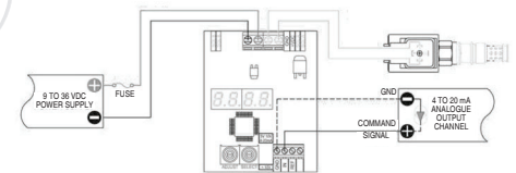
4) EXTERNAL INPUT SIGNAL CONNECTION 4-20 mA (in" set to "420")
