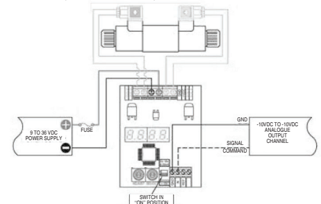
3) EXTERNAL INPUT SIGNAL CONNECTION (in" set to "10")
