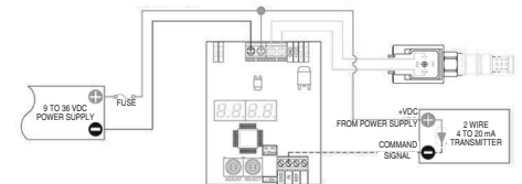
5) TWO WIRE TRANSMITTER INPUT CONNECTION 4-20 mA (in" set to "420")
