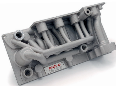
Hydraulic Manifold
