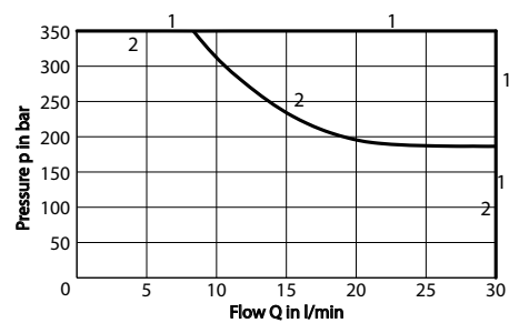
Hydraulic limits of use High performance valve
